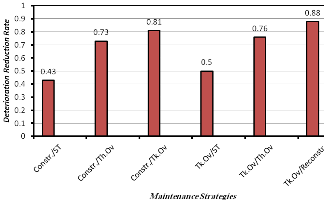
Figure 4: DRR for consecutive of different maintenance alternatives
