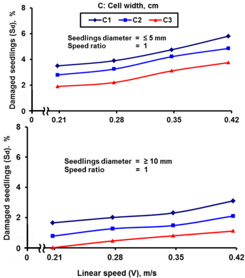
Figure (8): Effect of linear speed and cell width on damaged seedlings percentage at different Seedling diameters.
