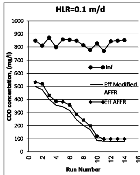
Fig (3-b) Start up results for COD Removal
