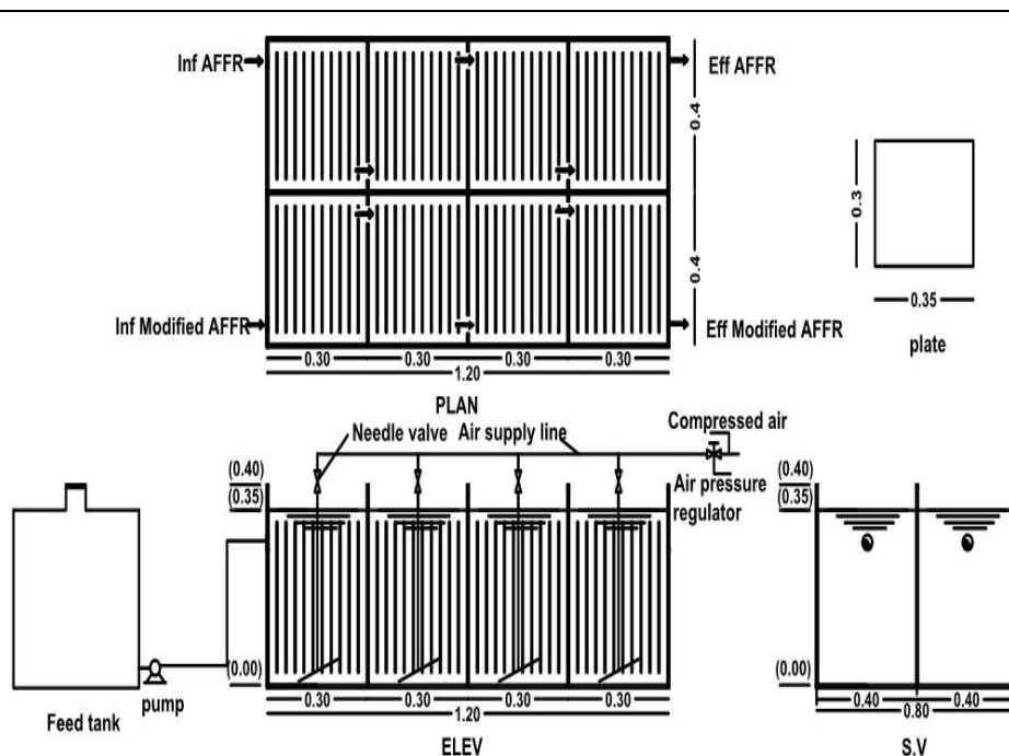
Fig (1) schematic diagram of AFFR's reactors
