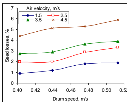
Fig. 9: The effect of drum speed on seed losses.
