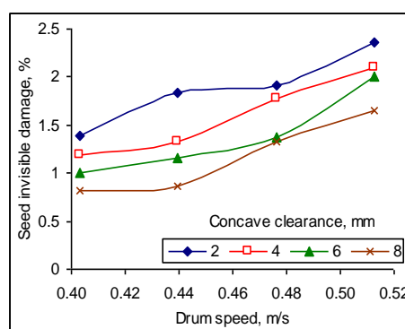
Fig. 5: The effect of drum speed seed invisible damage.
