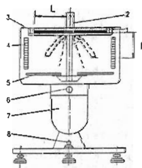
Fig. 5: Diagram of a flexometer for determining stiffness of fabrics at bending.
