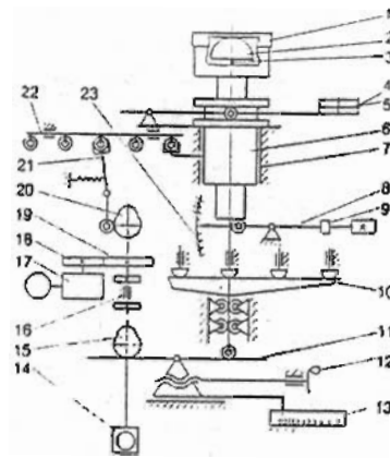
Fig. 1: Diagram of pulsator PD - 5M
