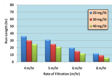
Figure 8: Run length versus filtration rate for 100 cm depth and C_o=20NTU .
