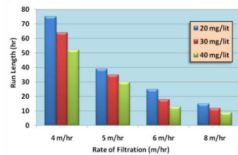
Figure 7: Run length versus filtration rate for 80 cm depth and C_o=20NTU .
