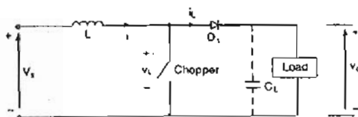
Figure 2 Step-up arrangement
