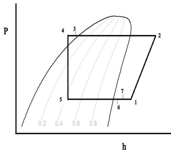
Fig. 2 P-h diagram for the system
