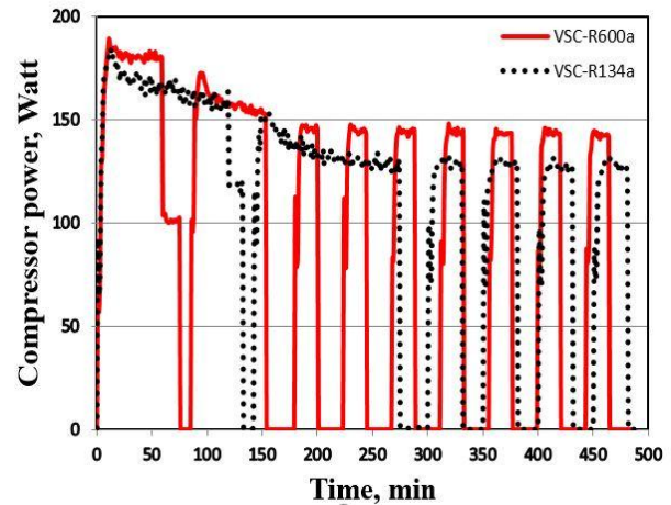
Fig. 10 Variation of the instantaneous power consumption of the variable speed compressor with the time
