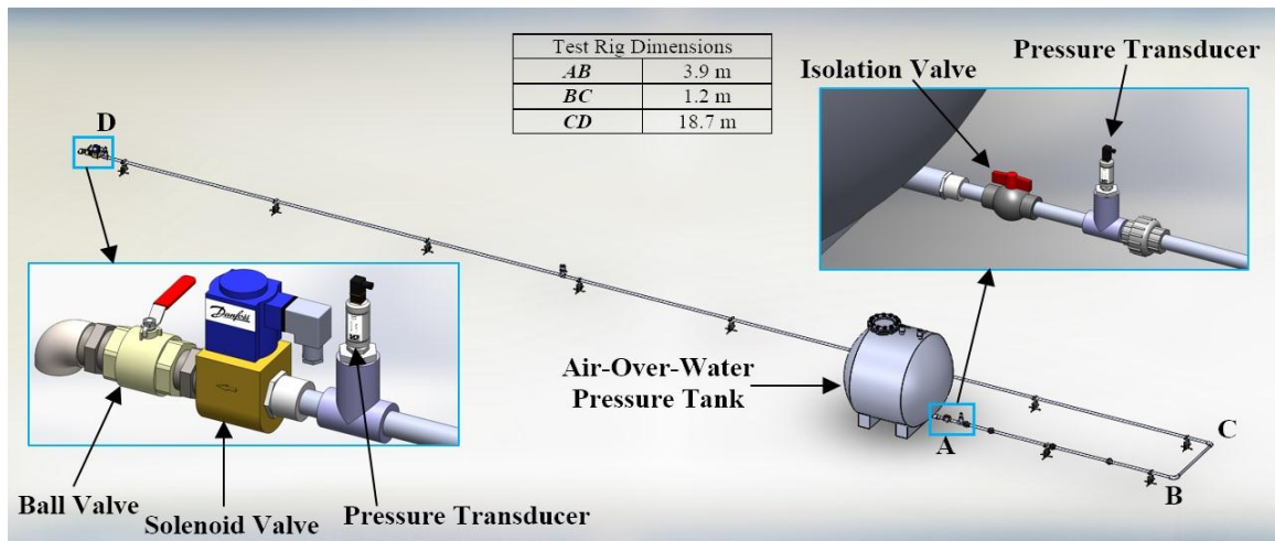
Fig. 5. Isometric view of water hammer test rig
