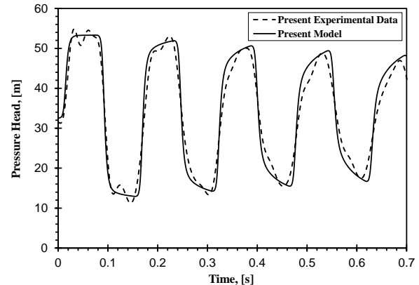
Fig. 11. Comparison between present model data and present experimental data at section M (Single pipe "Run S1")
