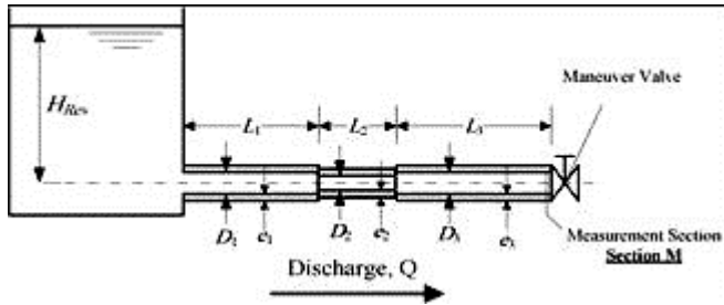
Fig. 8. Three pipes in series schematic diagram (Pipeline with extended blockage)
