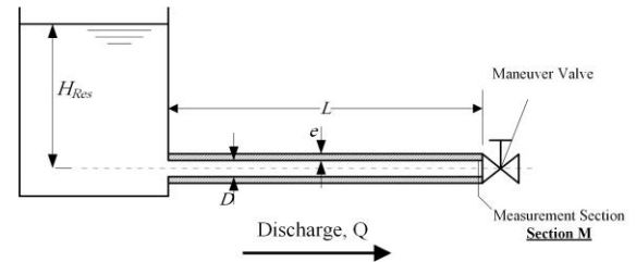
Fig. 7. Single pipe schematic diagram (Reservoir-Pipeline-Valve)
