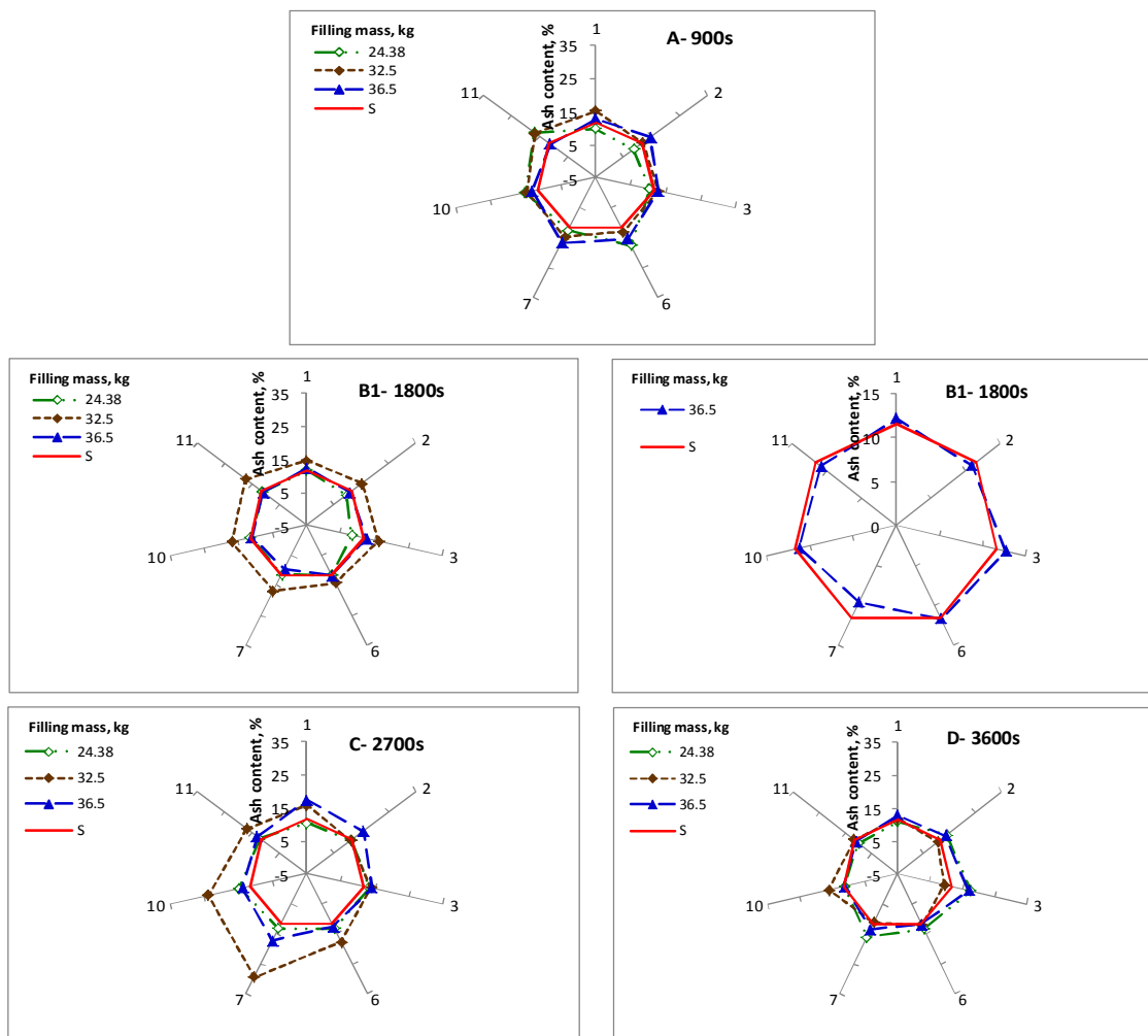
Fig. 6. The ash percentage at 25 rpm and different working times of 900; 1800; 2700 and 3600s
