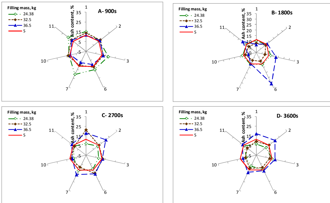
Fig. 8. The ash percentage at 45 rpm and different working times of 900; 1800; 2700 and 3600s
