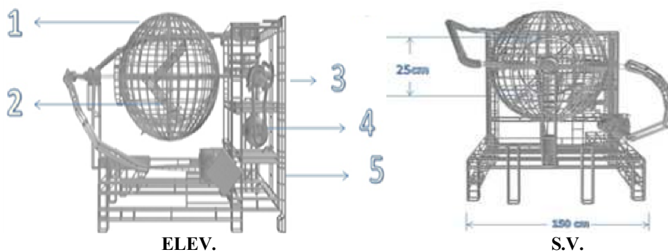
Fig. 1. Spherical mixer components
