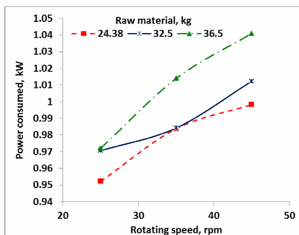
Fig. 9. The mixing consumption power at different raw material mass
