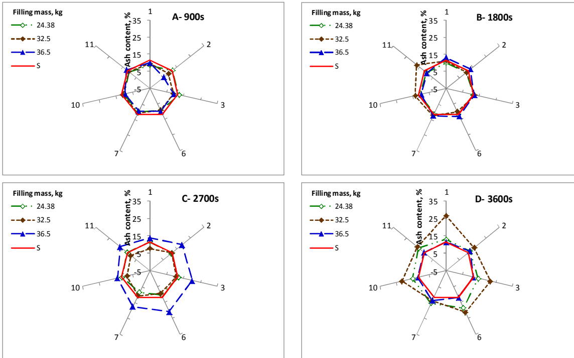
Fig. 7. The ash percentage at 35 rpm and different working times of 900; 1800; 2700 and 3600s
