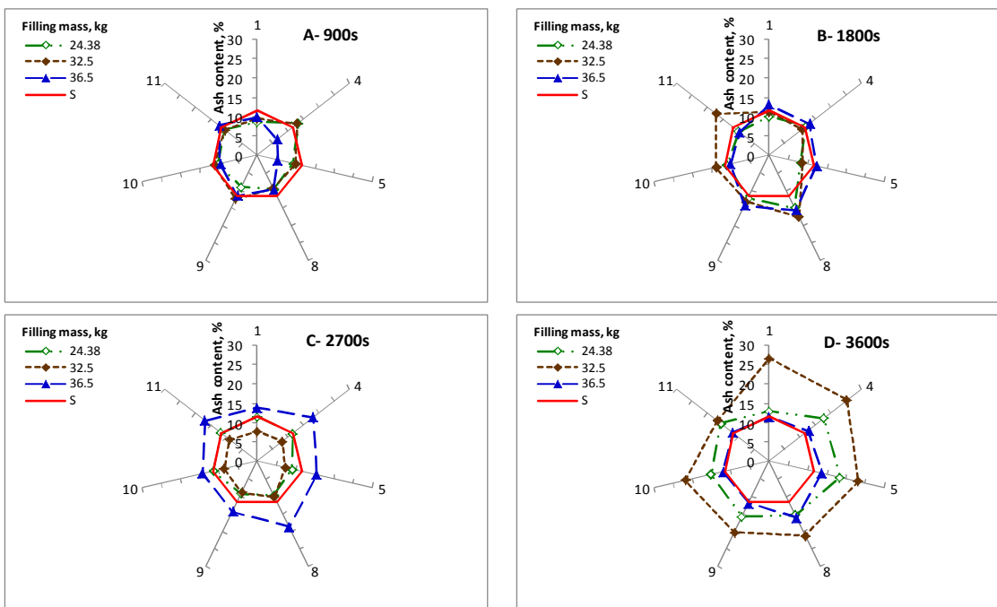
Fig. 4. The ash percentage at 35 rpm and different working times of 900; 1800; 2700 and 3600s
