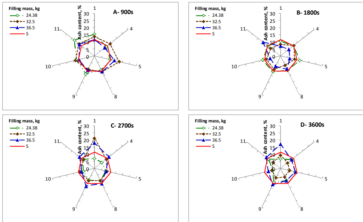
Fig. 5. The ash percentage at 45 rpm and different working times of 900; 1800; 2700 and 3600s
