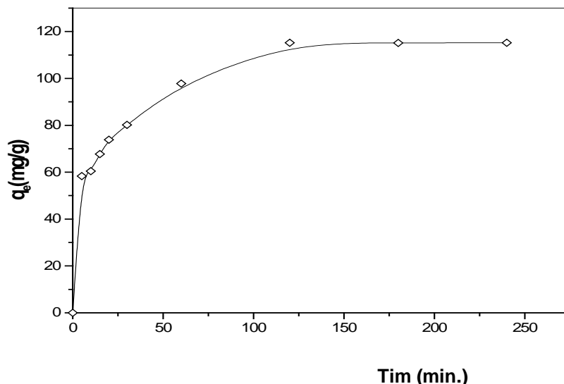
Fig. (1): Effect of time on adsorption of lead by MRH
