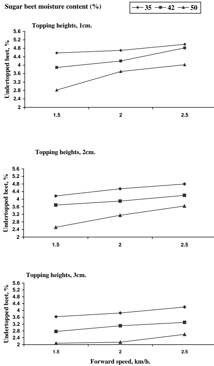
Fig.8.: Effect of forward speed and sugar beet moisture content on Undertopped beet percentage at topping heights 1,2 and 3 cm.
